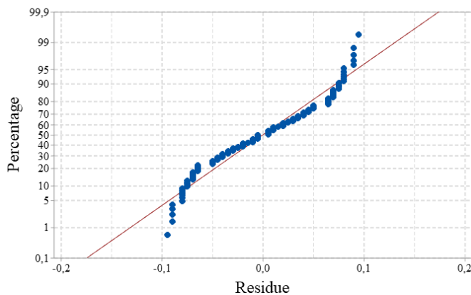
Fig. 15. Normal probability plot for the efficiency of the prototype II. Source:
