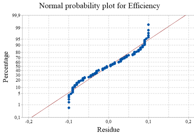
Fig. 9. Normal probability plot for the efficiency of the prototype I. Source: Own
